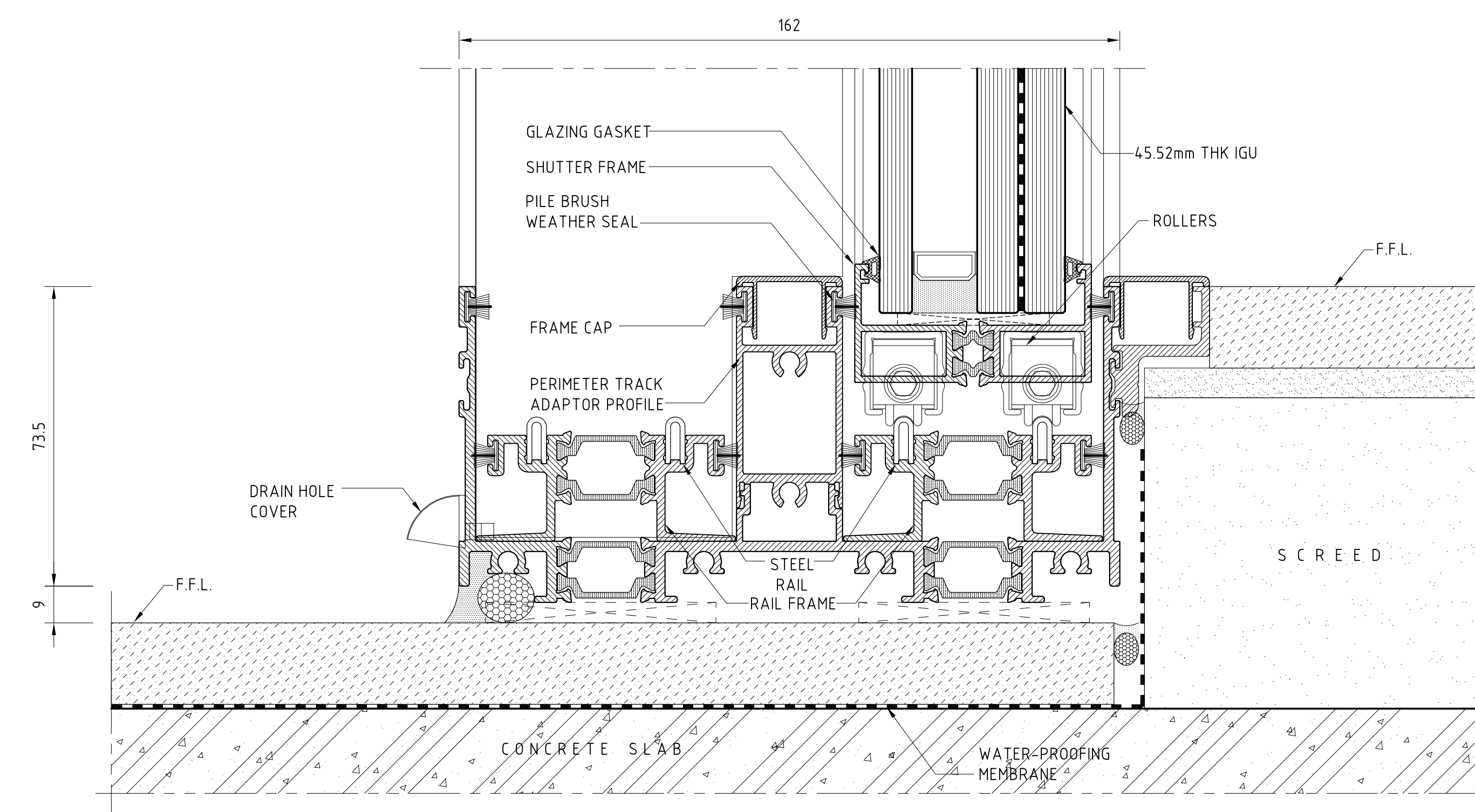
BOTTOM RAIL DETAIL
